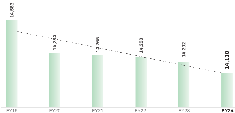
DC ENERGY (kWh/MT)
